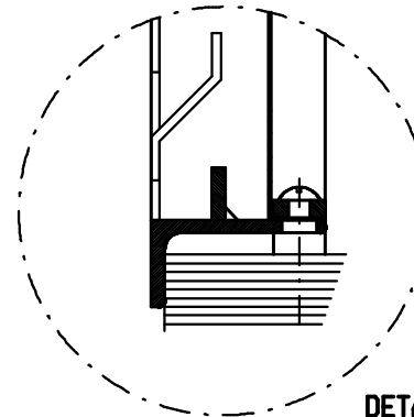
DETAIL E LAMELLEN STRIP 40x2 mm SCHAAL 1:1
